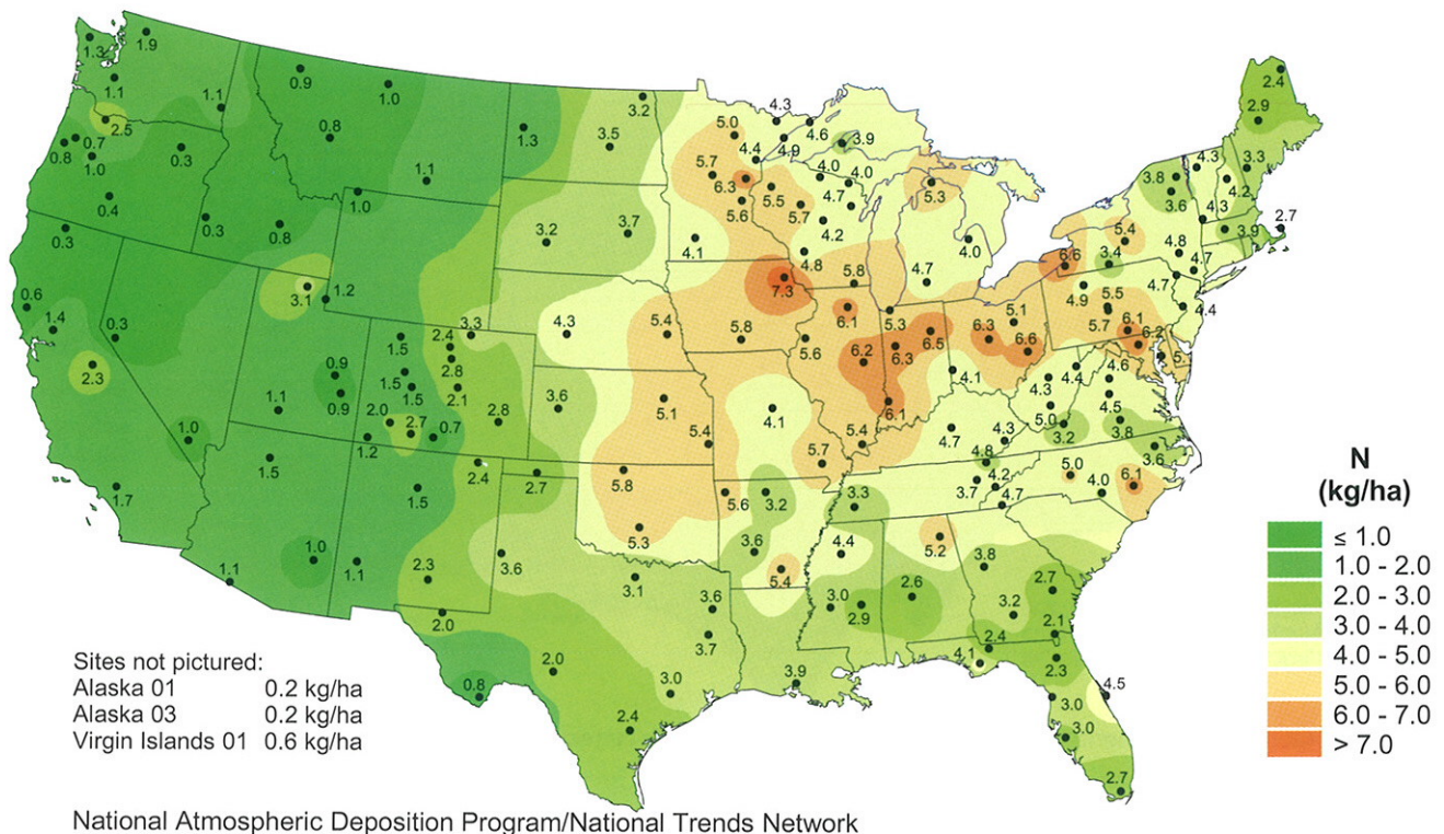
Estimated inorganic nitrogen deposition from nitrate and ammonium, 1999.
