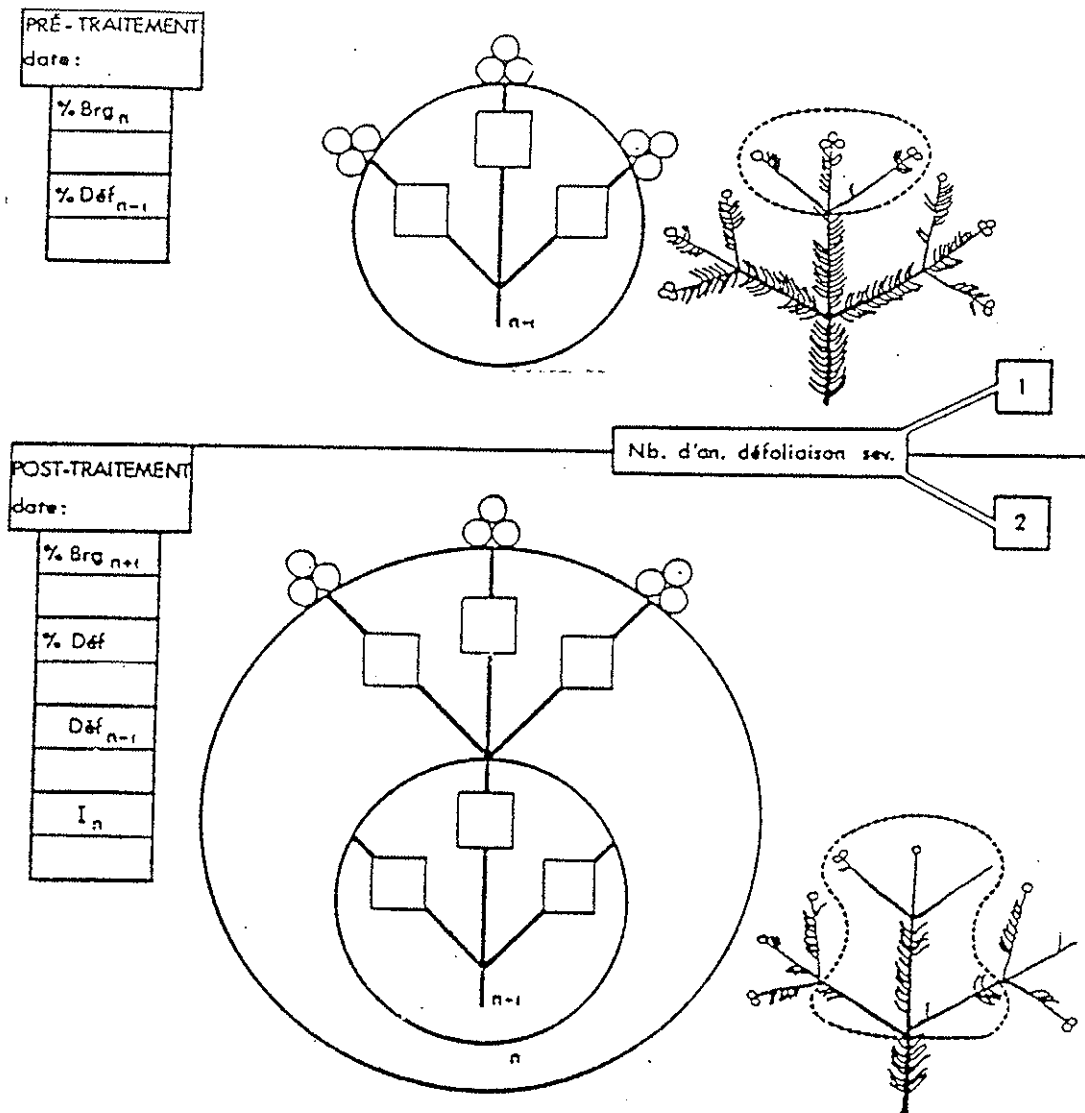
Figure 4. Method of estimating defoliation after Dorais and Hardy (1976) (From Sanders, 1980).
