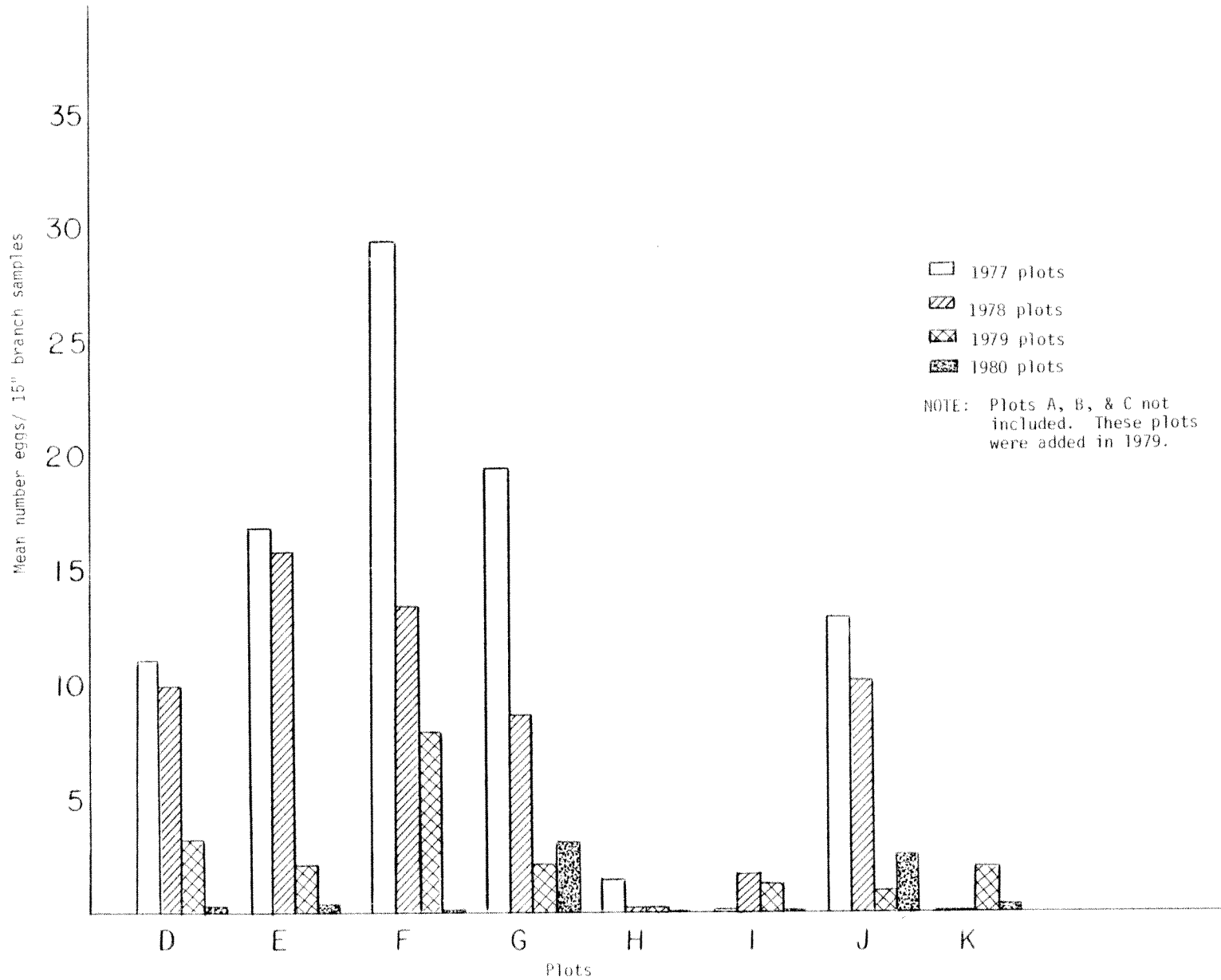
Figure 1-- Mean number eggs of oak leaftier per 15 inch branch samples per plot in 1977, 1978, 1979, & 1980
