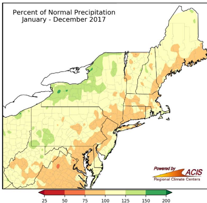
Figure 19. Across the 12 state region, the northeast saw below-average precipitation in 2017. Figure credit: NOAA, Northeast Regional Climate Center at Cornell University ( http://www.nrcc.cornell.edu/regional/monthly/monthly.html ).
