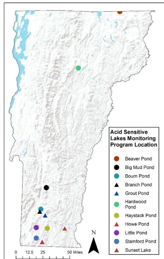
Figure 34. Locations of lakes/ponds in the Acid Lakes Monitoring Program in Vermont.
